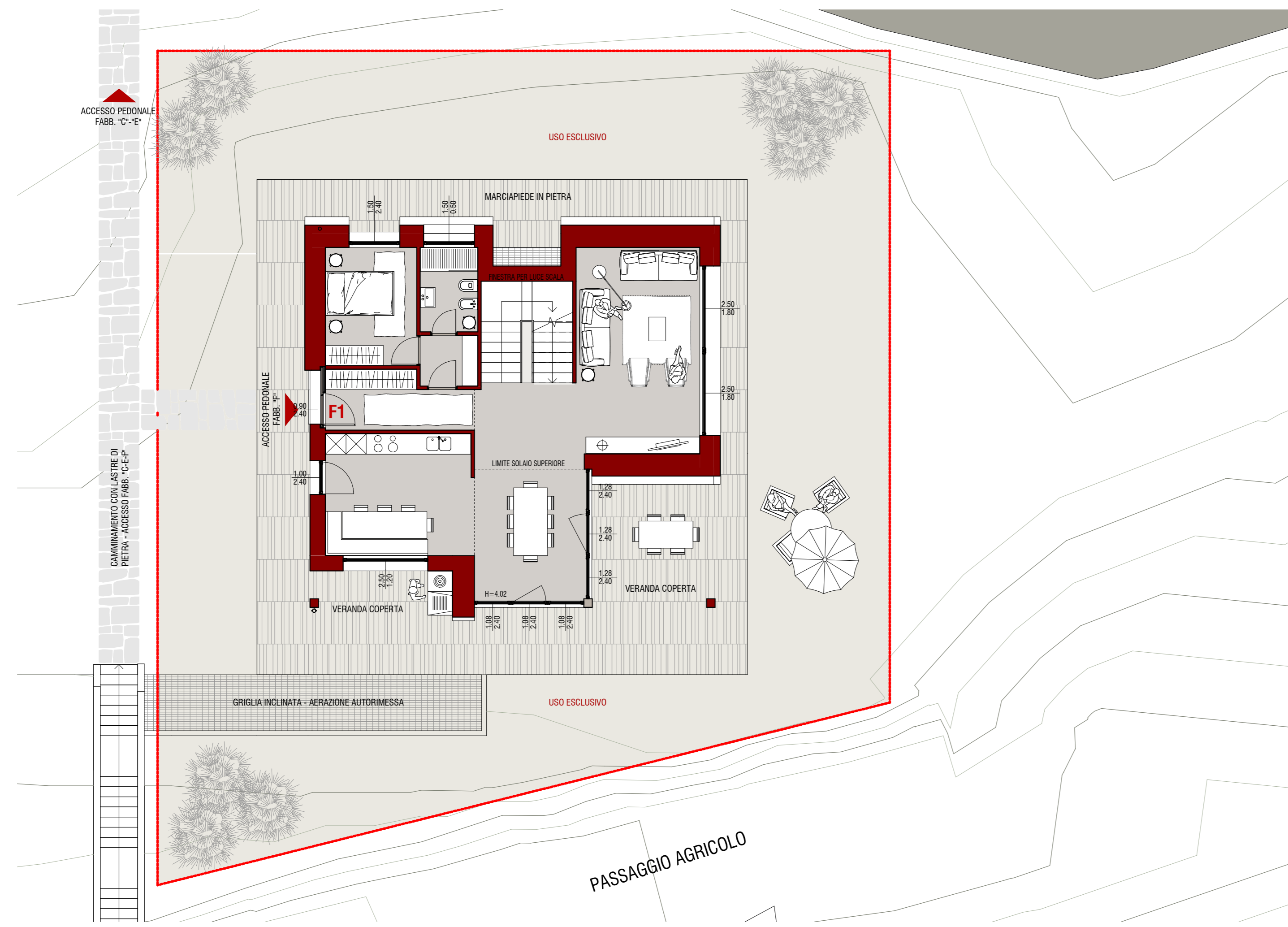
PIANO TERRA FAB. "F" 1 : 100
